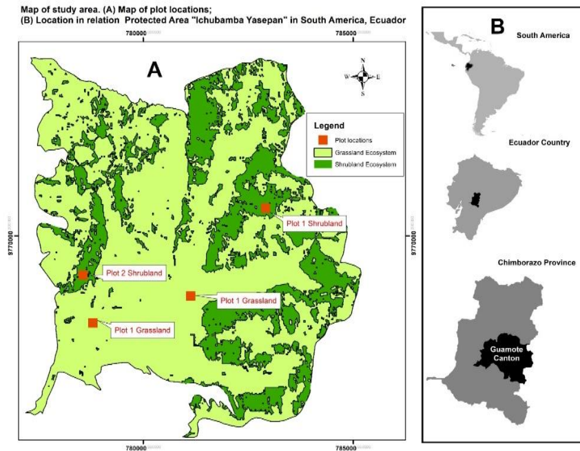
Figure 1. Location of the study area in the moors of the protected area "Ichubamba Yasepan", of the herbazal and shrub ecosystems 4 plots were installed.
