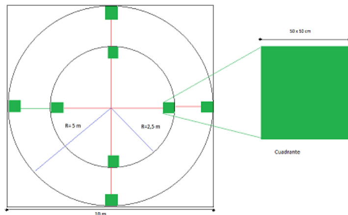
Figure 2. Plot design, subplots and quadrants for random cross data collection
