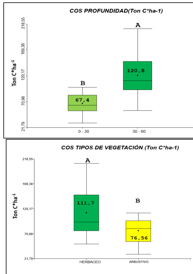
Figure 6. Carbon content at soil depth and vegetation types
