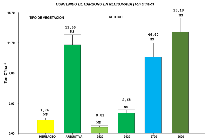
Figure 3. Carbon content in necromass according to the type of herbaceous and shrubby vegetation, and altitude
